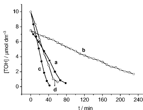
Figure 8. Decay of \alpha -tocopherol (TOH) during the inhibition of linoleic acid peroxidation in micelles at 37°C, initiated with AAPH and inhibited with TOH and quercetin (Q). a) Decay of TOH in the absence of Q in SDS micelles ( 0.1 \text{ mol L}^{-1} ), b) decay of TOH in the presence of Q in SDS micelles ( 0.1 \text{ mol L}^{-1} ), c) decay of TOH in the absence of Q in CTAB micelles ( 15 \text{ mmol L}^{-1} ), d) decay of TOH in the presence of Q in CTAB micelles ( 15 \text{ mmol L}^{-1} ). [LH]_0 = 15.2 \text{ mmol L}^{-1} , [AAPH]_0 = 6.3 \text{ mmol L}^{-1} , [TOH]_0 = 7.5 \text{ } \mu\text{mol L}^{-1} (SDS), [TOH]_0 = 10 \text{ } \mu\text{mol L}^{-1} (CTAB), [Q]_0 = 10 \text{ } \mu\text{mol L}^{-1} .
