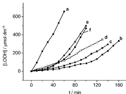
Figure 4. Representative kinetic curves for the formation of total hydroperoxides (LOOH) during the peroxidation of linoleic acid (LH) in CTAB micelles ( 15 \text{ mmol L}^{-1} ) at pH 7.4 and 37^\circ\text{C} , initiated with AAPH and inhibited by flavonols and their glycosides (FOHs). [\text{LH}]_0 = 15.2 \text{ mmol L}^{-1} , [\text{AAPH}]_0 = 6.3 \text{ mmol L}^{-1} , [\text{FOHs}]_0 = 10 \text{ μmol L}^{-1} . a) Uninhibited peroxidation, b) reaction inhibited with MY, c) reaction inhibited with Q, d) reaction inhibited with QG, e) reaction inhibited with MO, f) reaction inhibited with K. Curves of other FOHs are not shown for clarity.
