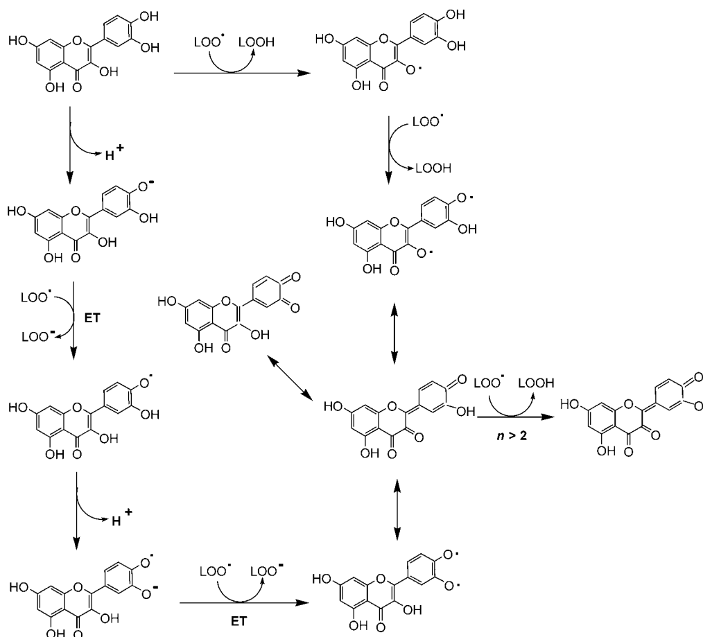
Scheme 2. Antioxidation reactions of quercetin (Q) by hydrogen abstraction and electron transfer.
