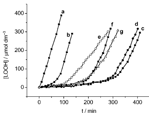
Figure 5. Representative kinetic curves for the formation of total hydroperoxides (LOOH) during the peroxidation of linoleic acid (LH) in SDS micelles ( 0.1 \text{ mol L}^{-1} ) at pH 7.4 and 37^\circ\text{C} , initiated with AAPH and inhibited with TOH and FOHs. [\text{LH}]_0 = 15.2 \text{ mmol L}^{-1} , [\text{AAPH}]_0 = 6.3 \text{ mmol L}^{-1} , [\text{FOHs}]_0 = 10 \text{ μmol L}^{-1} , [\text{TOH}]_0 = 7.5 \text{ μmol L}^{-1} . a) Uninhibited peroxidation, b) reaction inhibited with TOH, c) reaction inhibited with MY and TOH, d) reaction inhibited with Q and TOH, e) reaction inhibited with QG and TOH, f) reaction inhibited with MO and TOH, g) reaction inhibited with K and TOH. Curves of other FOHs are not shown for clarity.
