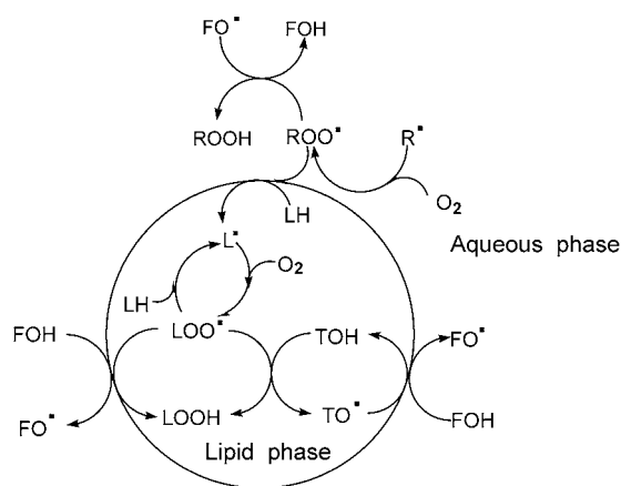
Scheme 1. Antioxidative and TOH-regeneration reactions of FOH in micelles.
