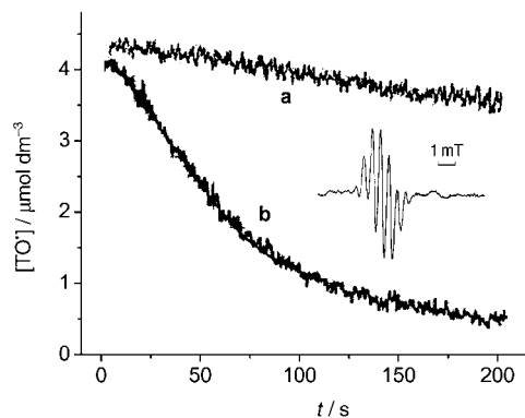
Figure 9. Decay of \alpha -tocopheroxyl radical ( TO^\bullet ) in SDS micelles ( 0.2 \text{ mol L}^{-1} ) at pH 7.4 and room temperature under air in the absence (a) and presence (b) of quercetin ( 0.21 \text{ mmol L}^{-1} ). The inset shows the EPR spectrum of TO^\bullet obtained under fast flow.
