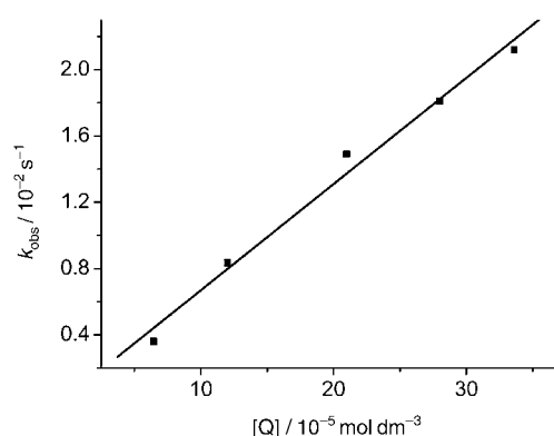
Figure 10. Plot of the pseudo-first-order rate constants, k_{\text{obs}} , of the decay of TO^\bullet versus the initial concentration of quercetin in SDS micelles ( 0.2 \text{ mol L}^{-1} ).
