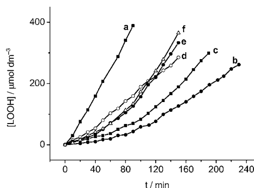
Figure 3. Representative kinetic curves for the formation of total hydroperoxides (LOOH) during the peroxidation of linoleic acid (LH) in SDS micelles ( 0.1 \text{ mol L}^{-1} ) at pH 7.4 and 37°C, initiated with AAPH and inhibited by flavonols and their glycosides (FOHs). [LH]_0 = 15.2 \text{ mmol L}^{-1} , [AAPH]_0 = 6.3 \text{ mmol L}^{-1} , [FOHs]_0 = 10 \text{ μmol L}^{-1} . a) Uninhibited peroxidation, b) reaction inhibited with MY, c) reaction inhibited with Q, d) reaction inhibited with QG, e) reaction inhibited with MO, f) reaction inhibited with K. Curves of other FOHs are not shown for clarity.
