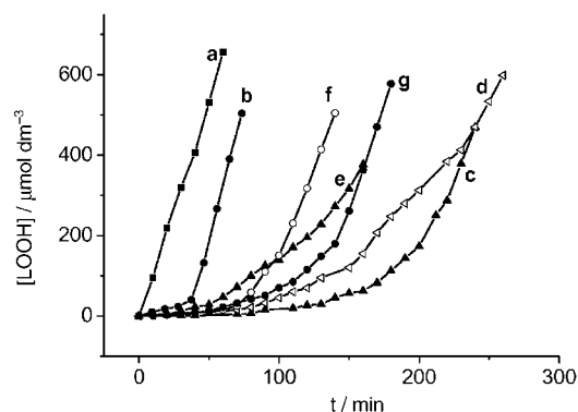
Figure 6. Representative kinetic curves for the formation of total hydroperoxides (LOOH) during the peroxidation of linoleic acid (LH) in CTAB micelles ( 15 \text{ mmol L}^{-1} ) at pH 7.4 and 37^\circ\text{C} , initiated with AAPH and inhibited with TOH and FOHs. [\text{LH}]_0 = 15.2 \text{ mmol L}^{-1} , [\text{AAPH}]_0 = 6.3 \text{ mmol L}^{-1} , [\text{FOHs}]_0 = 10 \text{ μmol L}^{-1} , [\text{TOH}]_0 = 10 \text{ μmol L}^{-1} . a) Uninhibited peroxidation, b) reaction inhibited with TOH, c) reaction inhibited with MY and TOH, d) reaction inhibited with Q and TOH, e) reaction inhibited with QG and TOH, f) reaction inhibited with MO and TOH, g) reaction inhibited with K and TOH. Curves of other FOHs are not shown for clarity.
