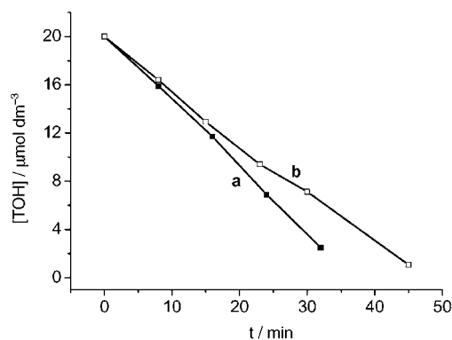
Figure 7. Decay of \alpha -tocopherol (TOH) during the inhibition of linoleic acid peroxidation in tert -butyl alcohol/water (3:2) solution at 37°C, initiated with AAPH and inhibited with TOH in the absence (a) and presence (b) of quercetin (Q). [LH]_0 = 0.1 \text{ mol L}^{-1} , [AAPH]_0 = 10 \text{ mmol L}^{-1} , [TOH]_0 = 20 \text{ } \mu\text{mol L}^{-1} , [Q]_0 = 20 \text{ } \mu\text{mol L}^{-1} .
