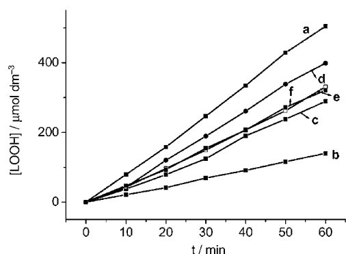
Figure 1. Representative kinetic curves for the formation of total hydroperoxides (LOOH) during the peroxidation of LH in tert -butyl alcohol/water (3:2) solution at 37°C, initiated with AAPH and inhibited with flavonols and their glycosides (FOHs). [LH]_0 = 0.1 \text{ mol L}^{-1} , [AAPH]_0 = 10 \text{ mmol L}^{-1} , [FOHs]_0 = 20 \text{ μmol L}^{-1} . a) Uninhibited reaction, b) reaction inhibited with MY, c) reaction inhibited with Q, d) reaction inhibited with QG, e) reaction inhibited with MO, f) reaction inhibited with K. Curves of other FOHs are not shown for clarity.
