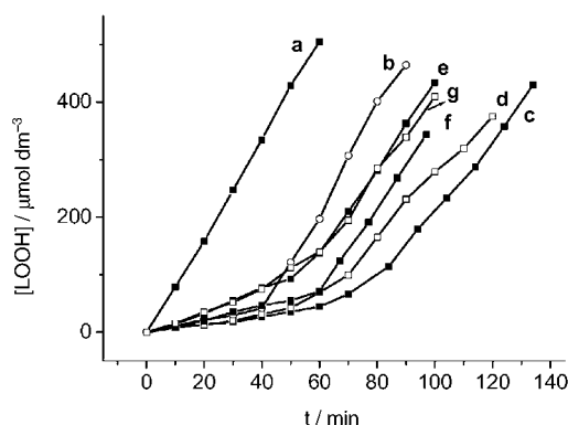
Figure 2. Representative kinetic curves for the formation of total hydroperoxides (LOOH) during the peroxidation of LH in tert -butyl alcohol/water (3:2) solution at 37°C, initiated with AAPH and inhibited with TOH and FOHs. [LH]_0 = 0.1 \text{ mol L}^{-1} , [AAPH]_0 = 10 \text{ mmol L}^{-1} , [TOH]_0 = 20 \text{ μmol L}^{-1} , [FOHs]_0 = 20 \text{ μmol L}^{-1} . a) Uninhibited reaction, b) reaction inhibited with TOH, c) reaction inhibited with MY and TOH, d) reaction inhibited with Q and TOH, e) reaction inhibited with QG and TOH, f) reaction inhibited with MO and TOH, g) reaction inhibited with K and TOH. Curves of other FOHs are not shown for clarity.
